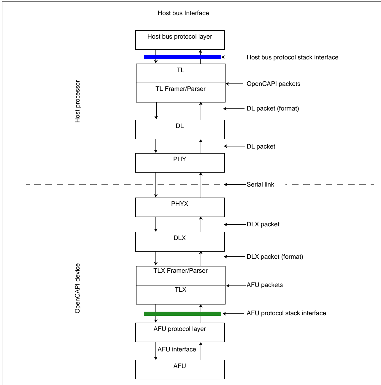
Figure 1-1. OpenCAPI stack
